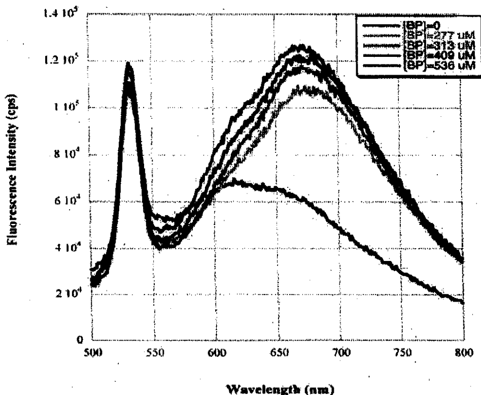
Fig. 4. Fluorescence spectra for complex from (13) using 475 nm excitation for [BP] = 0 and 277, 313, 409, 536 \mu M BP
